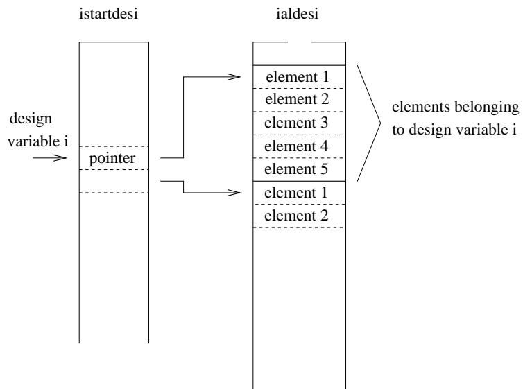
Figure 191: Data structure for all elements belonging to a specific design variable
