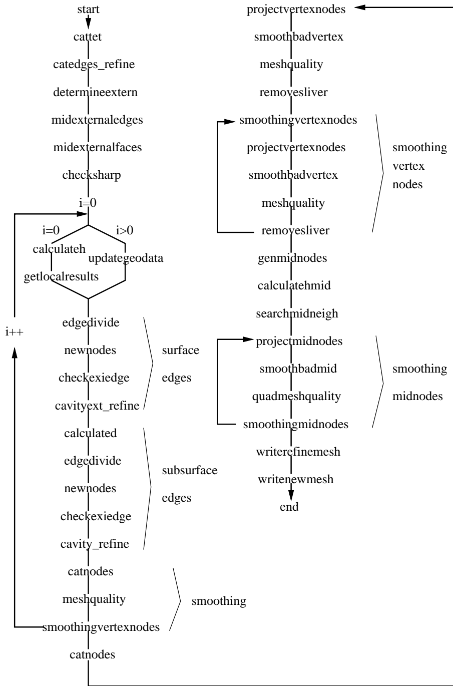
Figure 198: Flow diagram for mesh refinement
