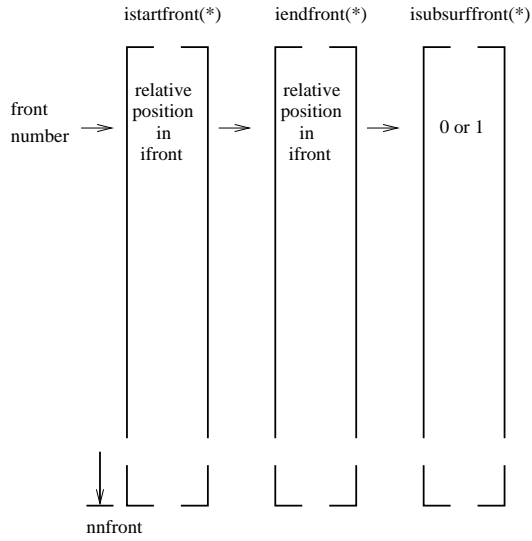
Figure 205: Fields for the front characteristics
