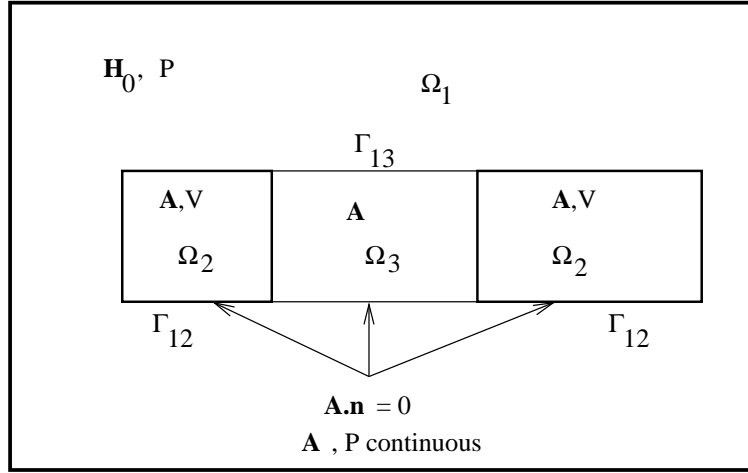
Figure 152: Electromagnetic setup for multiply connected bodies
