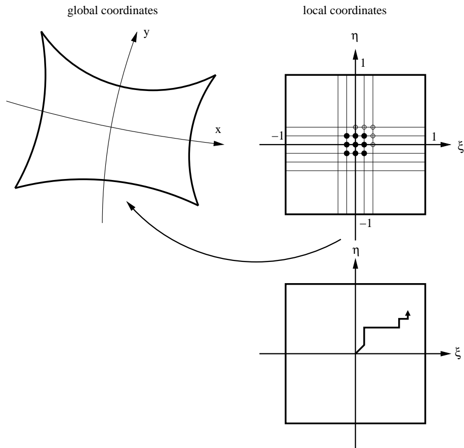
Figure 210: Closest location in an element
