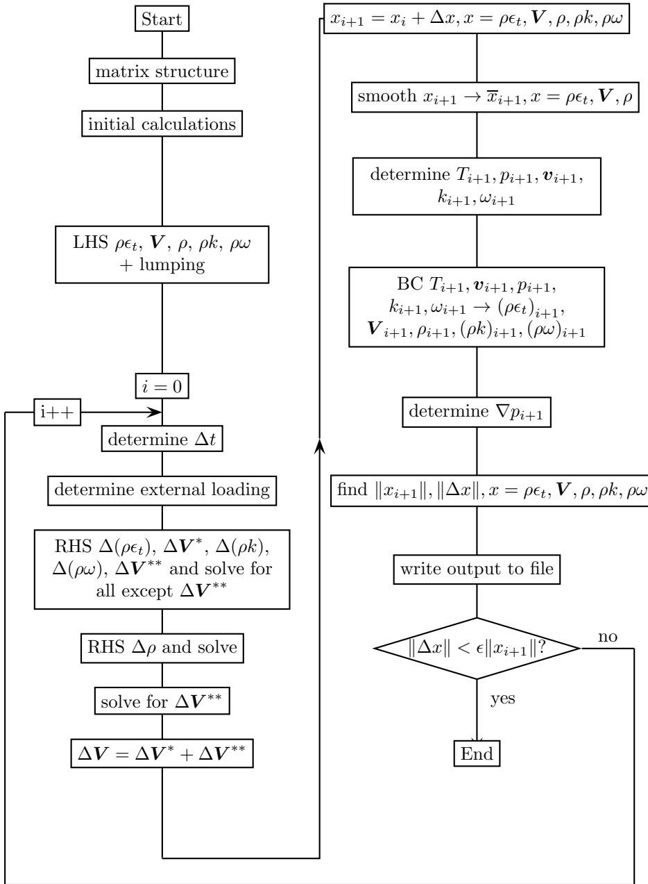
Figure 186: Flow diagram for compressible fluids
