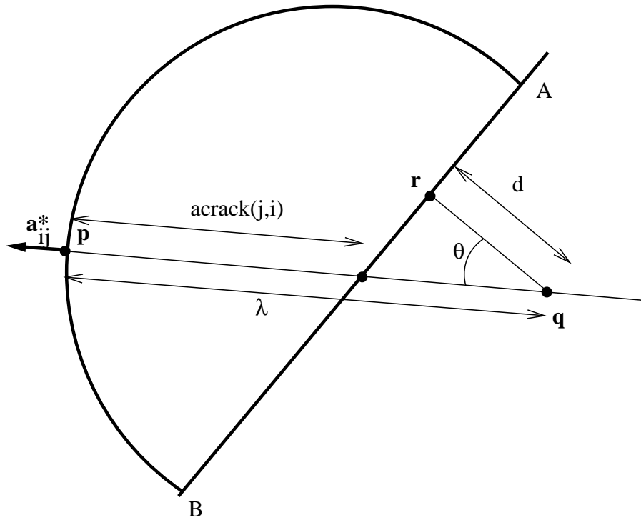
Figure 208: Calculation of the distance of a front node from the intersection of a straight line mit unit vector \mathbf{a}^* with the free surface
