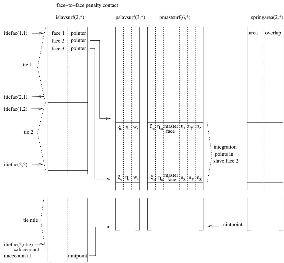
Figure 178: Storage of the slave faces (face-to-face penalty)
