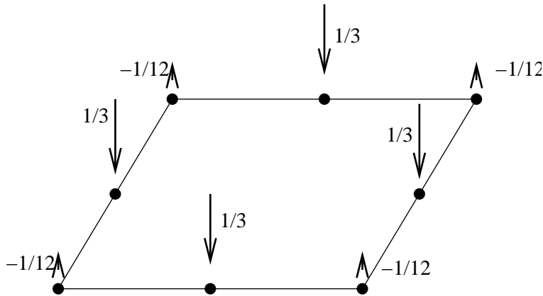
Figure 161: Equivalent forces of a uniform pressure on a plate (1 element)
