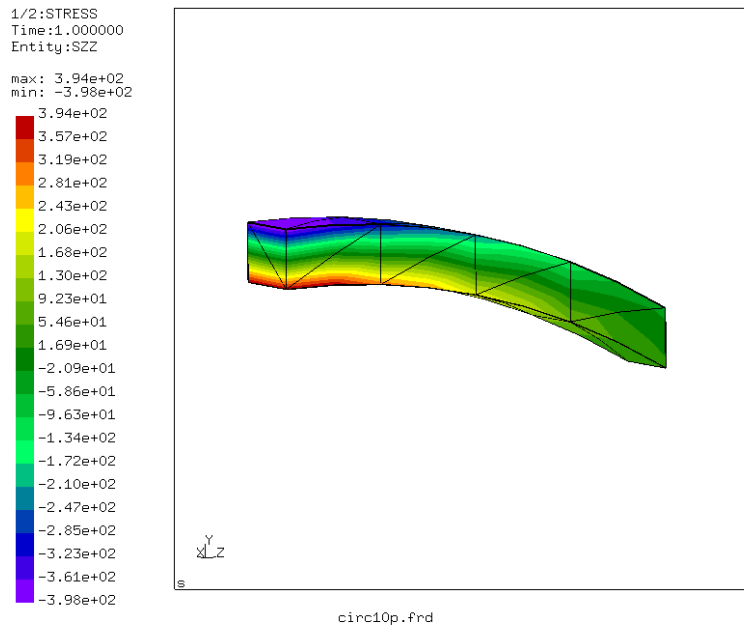
Figure 53: Normal stress in z-direction for the coarse mesh
