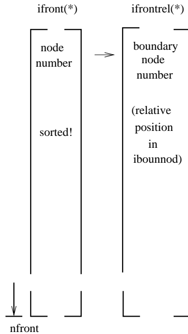
Figure 203: Fields for the front nodes (before analyzing the adjacency relations)
