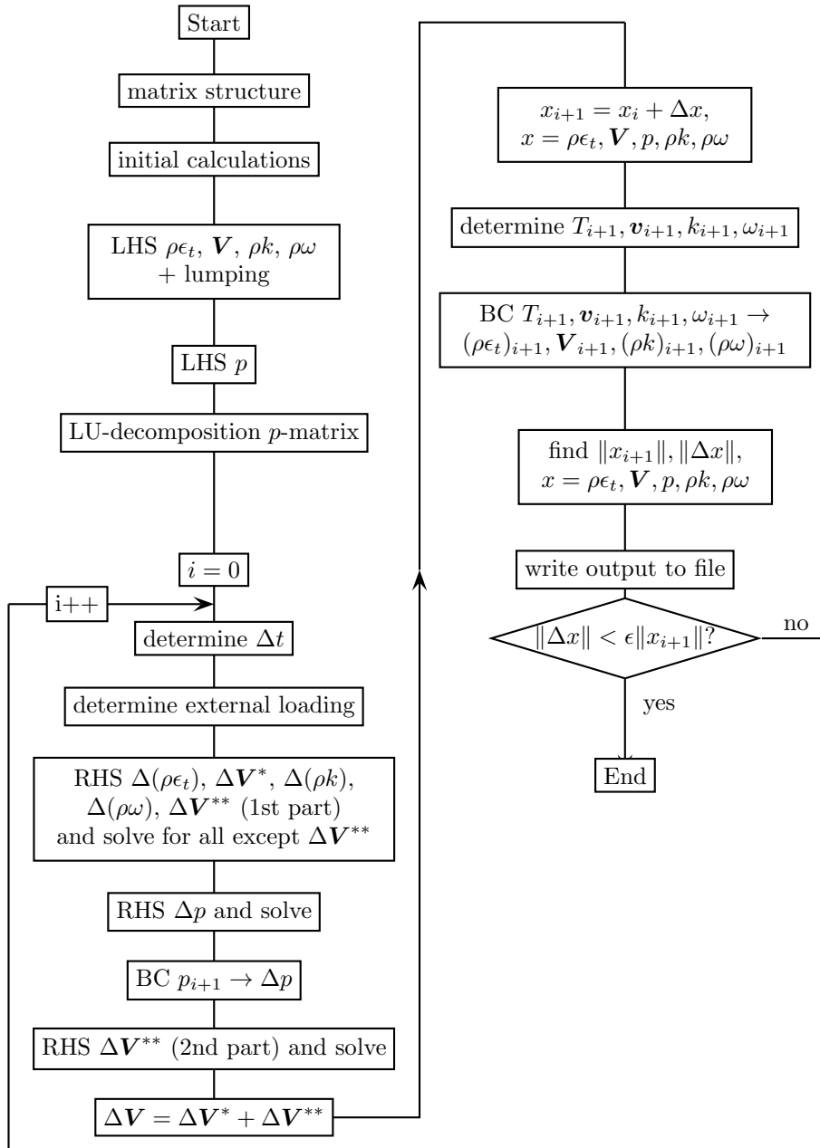
Figure 185: Flow diagram for liquids
