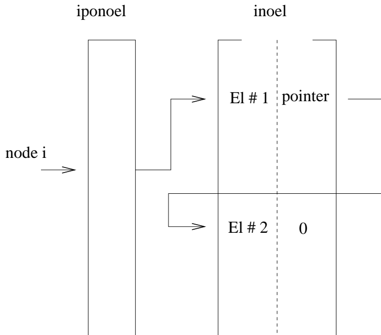
Figure 188: Data structure for all elements belonging to a given node
