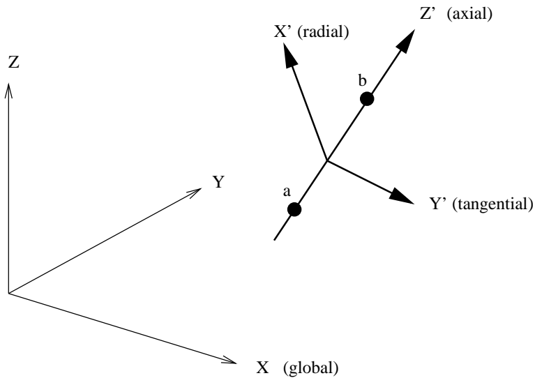
Figure 166: Definition of a cylindrical coordinate system
