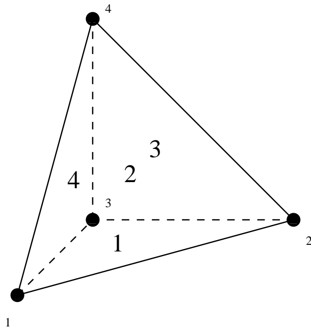
Figure 156: Face numbering for tetrahedral elements
