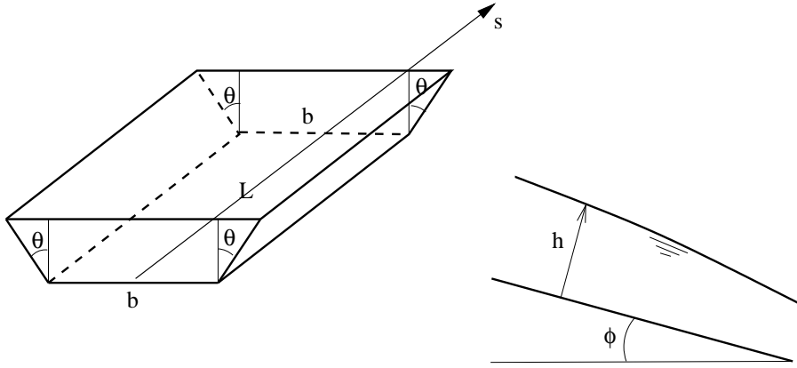
Figure 147: Channel geometry
