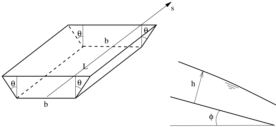
Figure 119: Channel geometry
