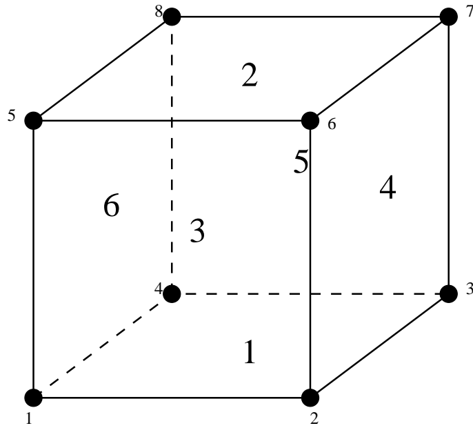
Figure 155: Face numbering for hexahedral elements
