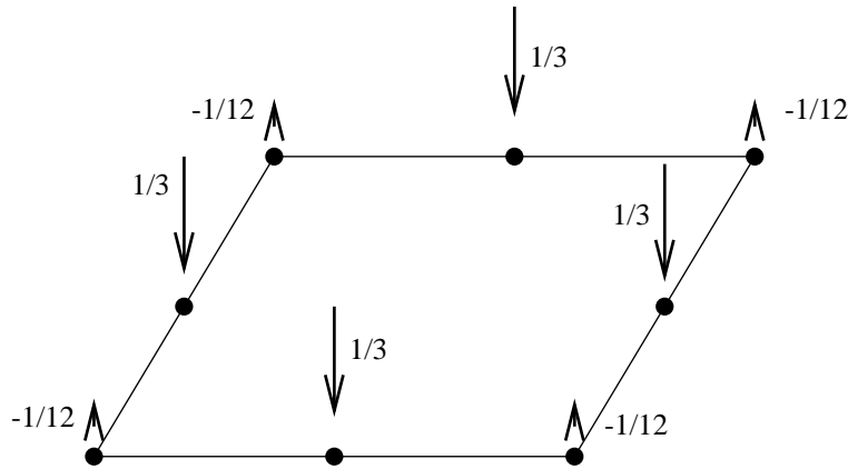
Figure 158: Equivalent nodal forces for a face of a C3D20(R) element
