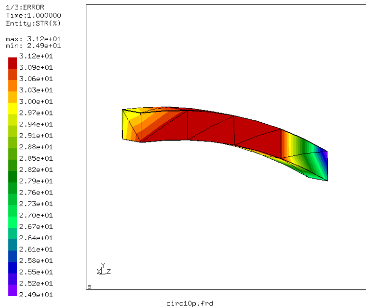
Figure 54: Error estimator for the coarse mesh
