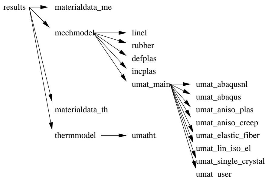
Figure 184: Flow diagram for subroutine results
