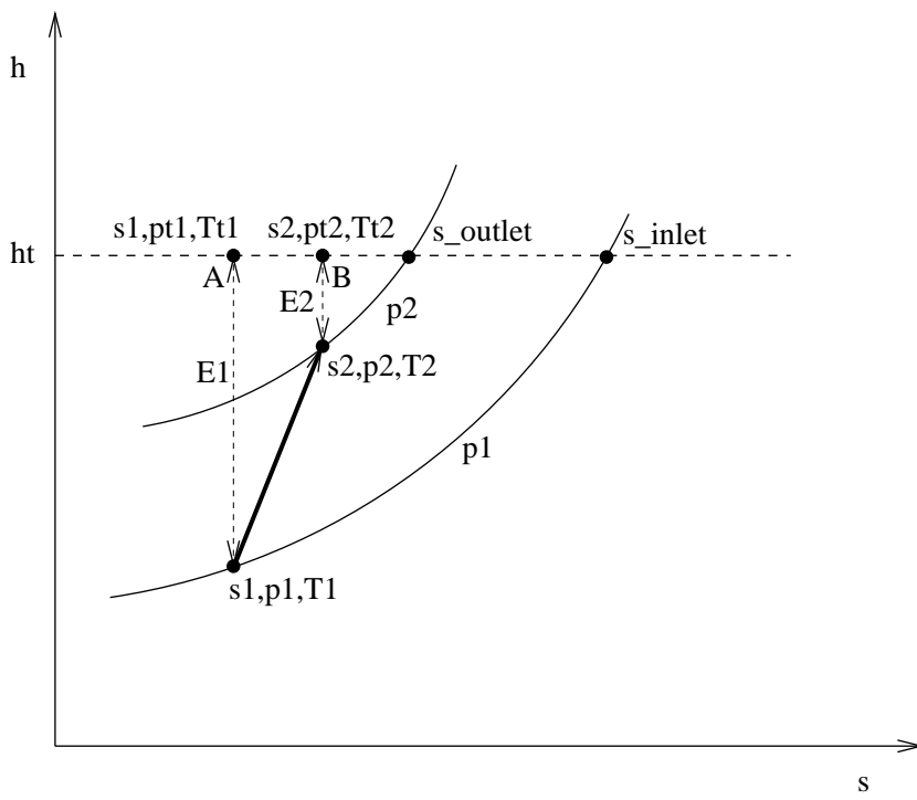
Figure 92: h-s diagram showing the restrictor process
