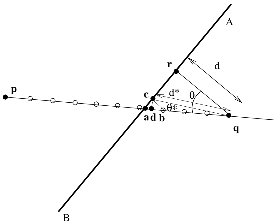
Figure 207: Calculation of a front position external but close to the free surface.
