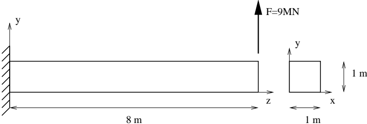
Figure 1: Geometry and boundary conditions of the beam problem
