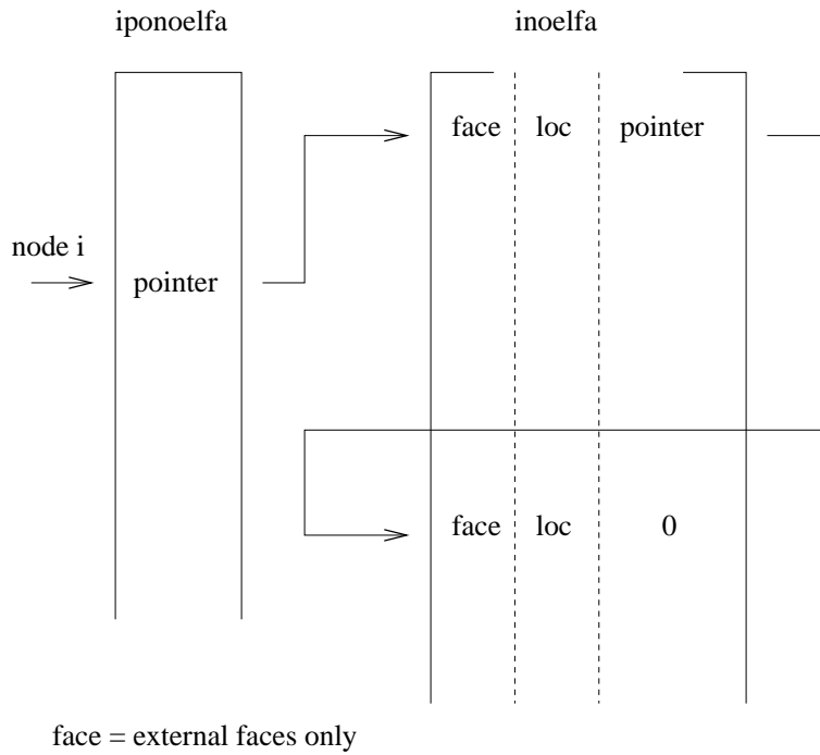
Figure 190: Data structure for all external faces belonging to a given node
