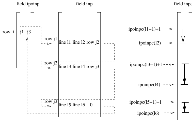
Figure 167: Reading the lines for keyword entry i
