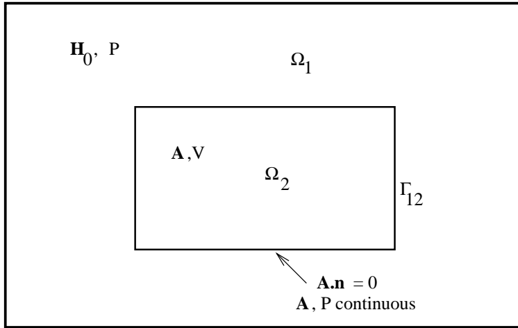
Figure 151: Electromagnetic setup for simply connected bodies
