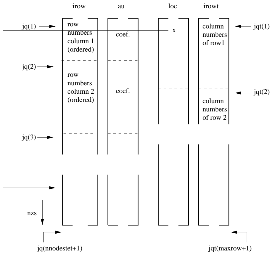
Figure 200: Fields describing the matrix structure
