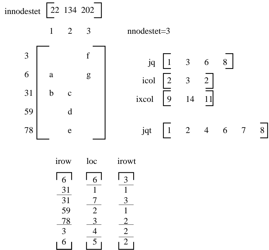
Figure 201: Example for the fields defining the connecting equations
