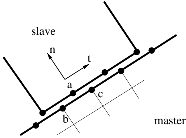
Figure 139: Contact area
