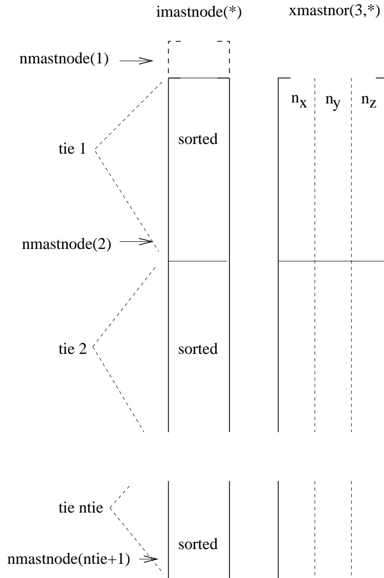
Figure 180: Storage of the master nodes
