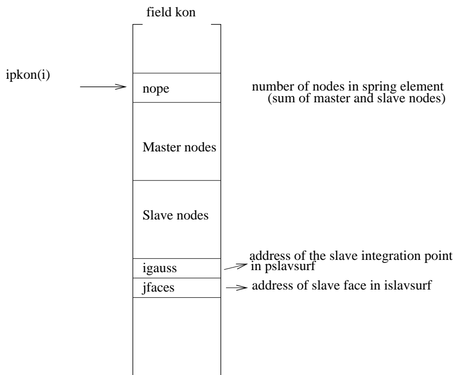
Figure 182: Topology of the face-to-face penalty contact elements
