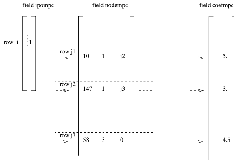
Figure 168: Example of the storage of a linear equation
