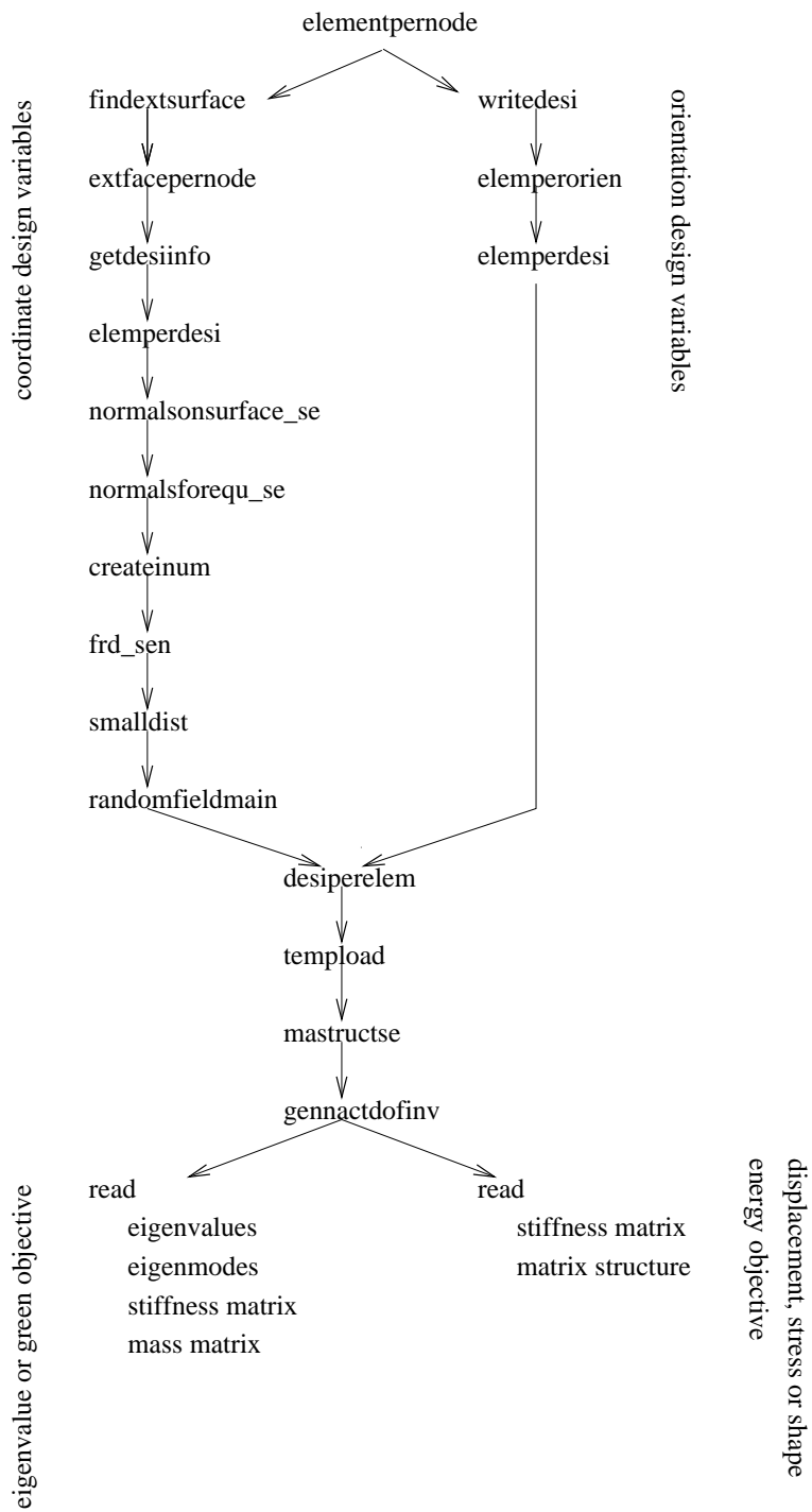
Figure 187: Structure of the preprocessing part
