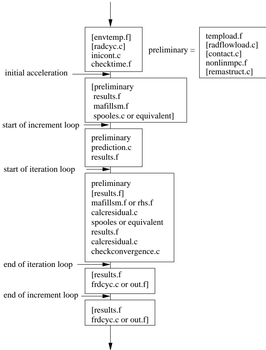
Figure 183: Flow diagram for subroutine nonlinge0
