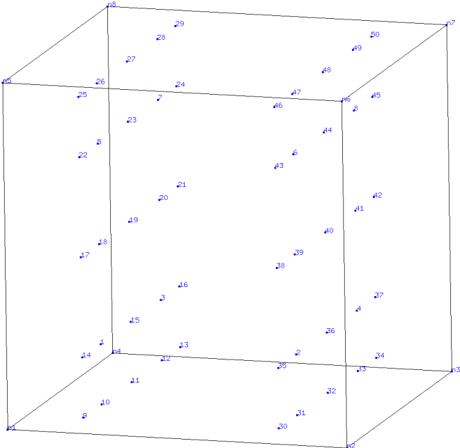
Figure 76: Gauss-Kronrod integration scheme for B32R elements with rectangular cross section
