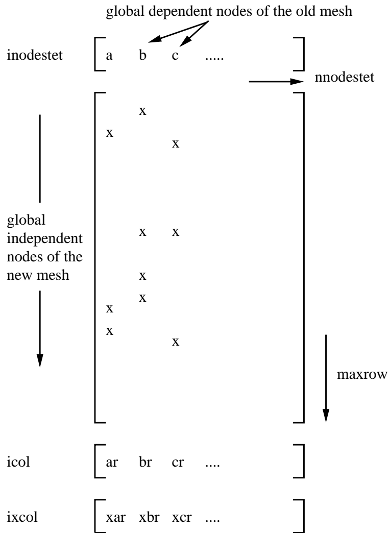
Figure 199: Matrix structure of the connecting equations
