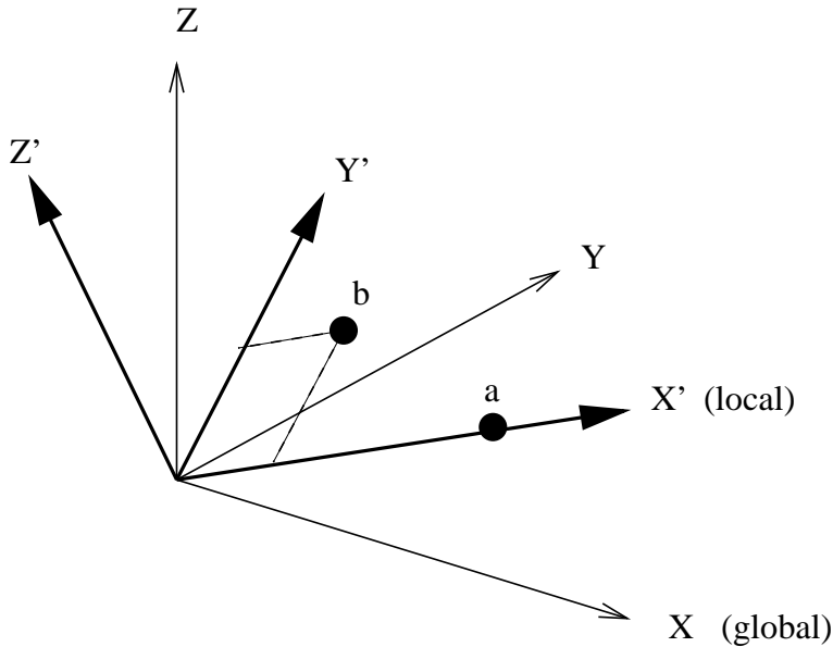
Figure 165: Definition of a rectangular coordinate system
