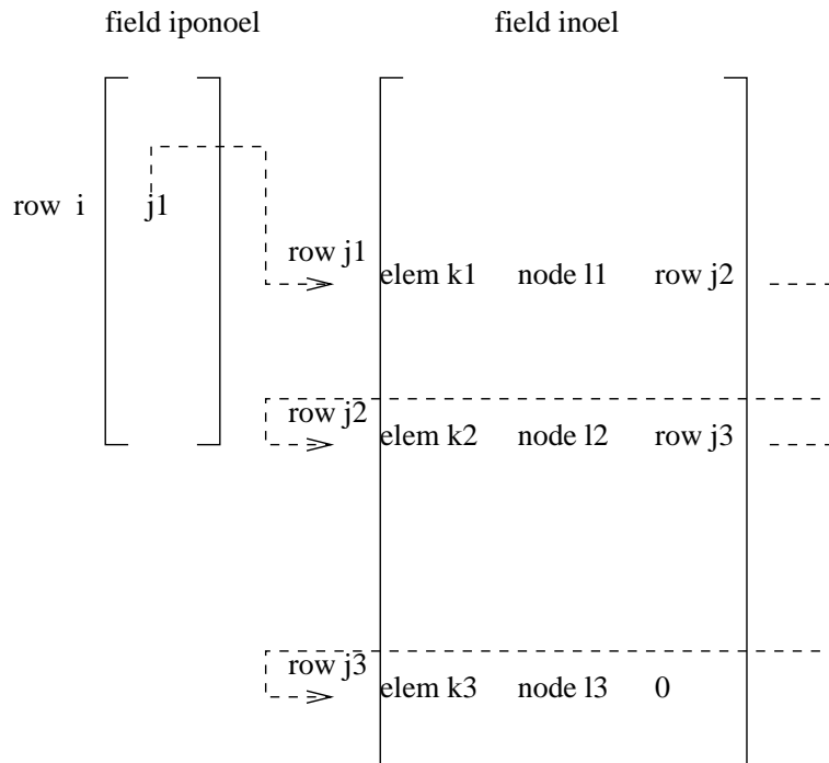
Figure 169: Structures to store all elements to which a given node belongs
