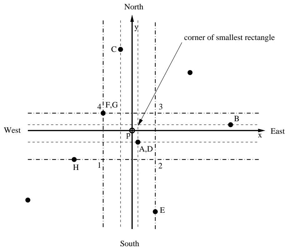
Figure 209: Scheme of the nearest point algorithm
