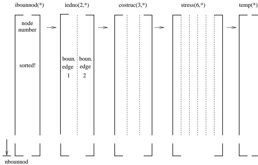
Figure 202: Fields for the boundary nodes and edges
