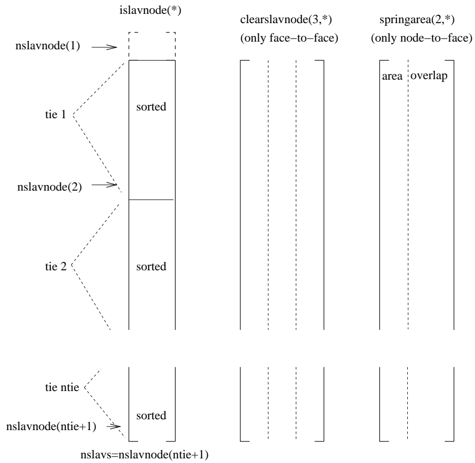
Figure 176: Storage of the slave nodes
