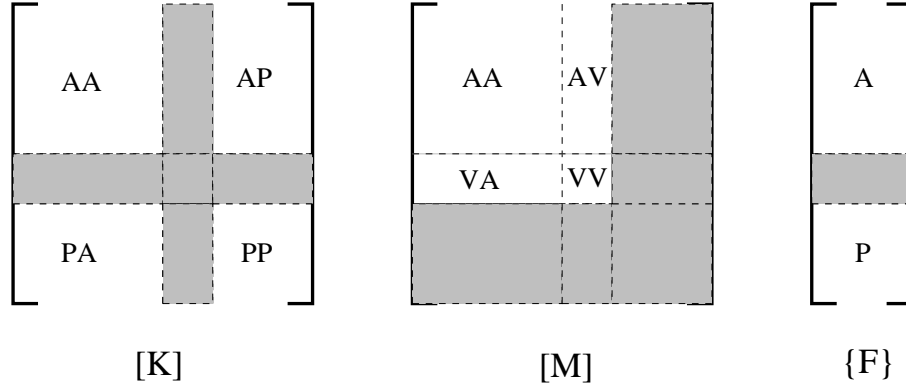
Figure 153: Nonzero parts of the governing matrices
