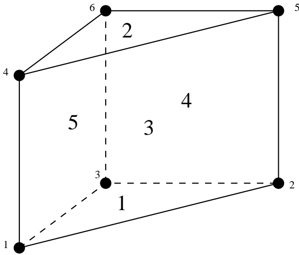
Figure 157: Face numbering for wedge elements
