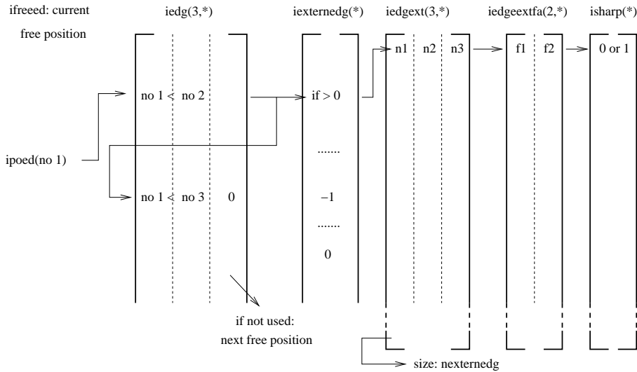
Figure 194: Node per edge relationship
