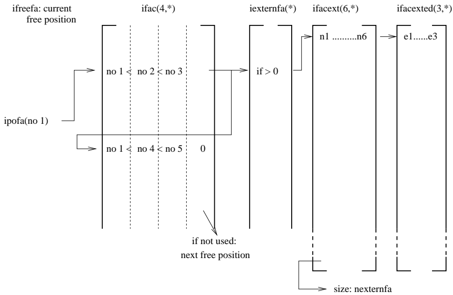
Figure 196: Node per face relationship
