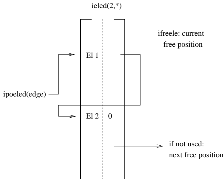
Figure 195: Element per edge relationship
