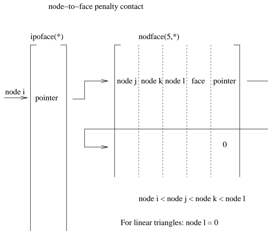
Figure 175: Storage of all faces for the determination of the external faces
