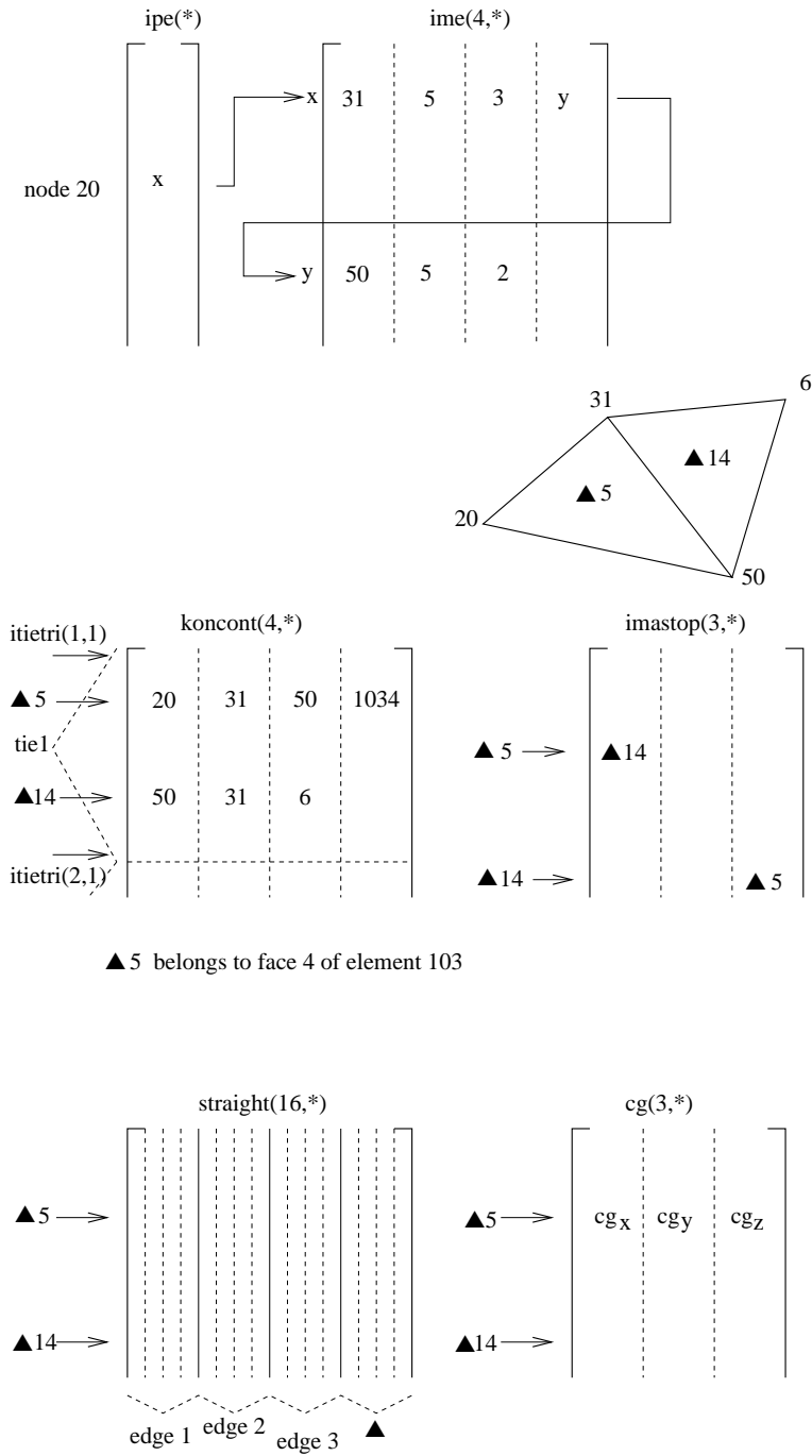
Figure 174: Storage of the triangulation properties
