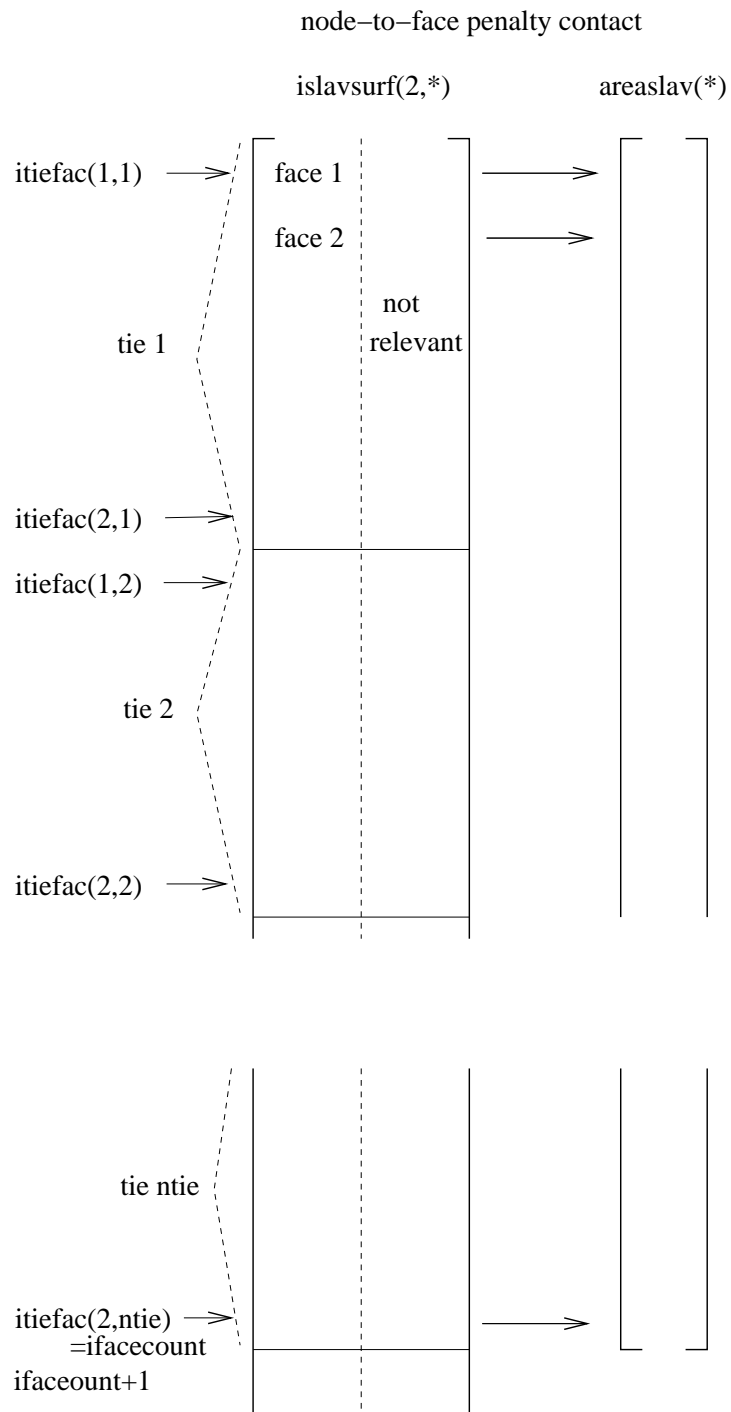
Figure 177: Storage of the slave faces (node-to-face penalty)
