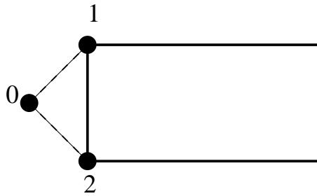
Figure 171: Shell element connection
