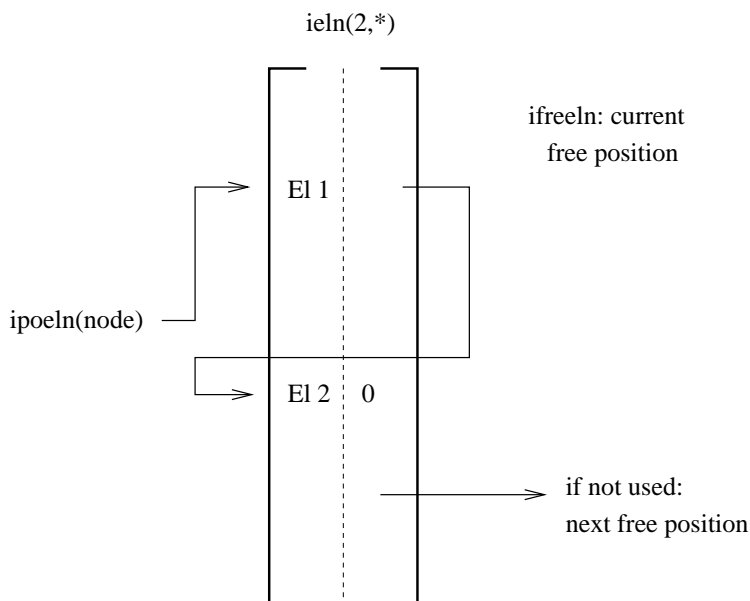
Figure 193: Element per node relationship
