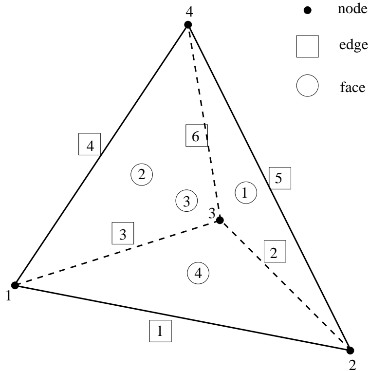
Figure 197: Node, edge and face numbering within a tetrahedral element
