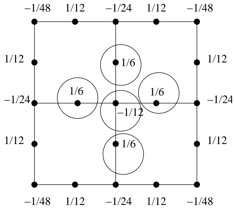
Figure 162: Equivalent forces of a uniform pressure on a plate (4 elements)
