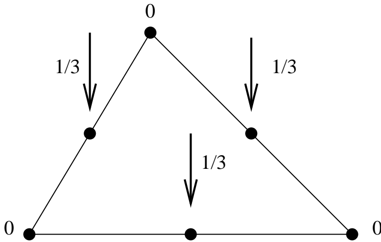
Figure 159: Equivalent nodal forces for a face of a C3D10 element
