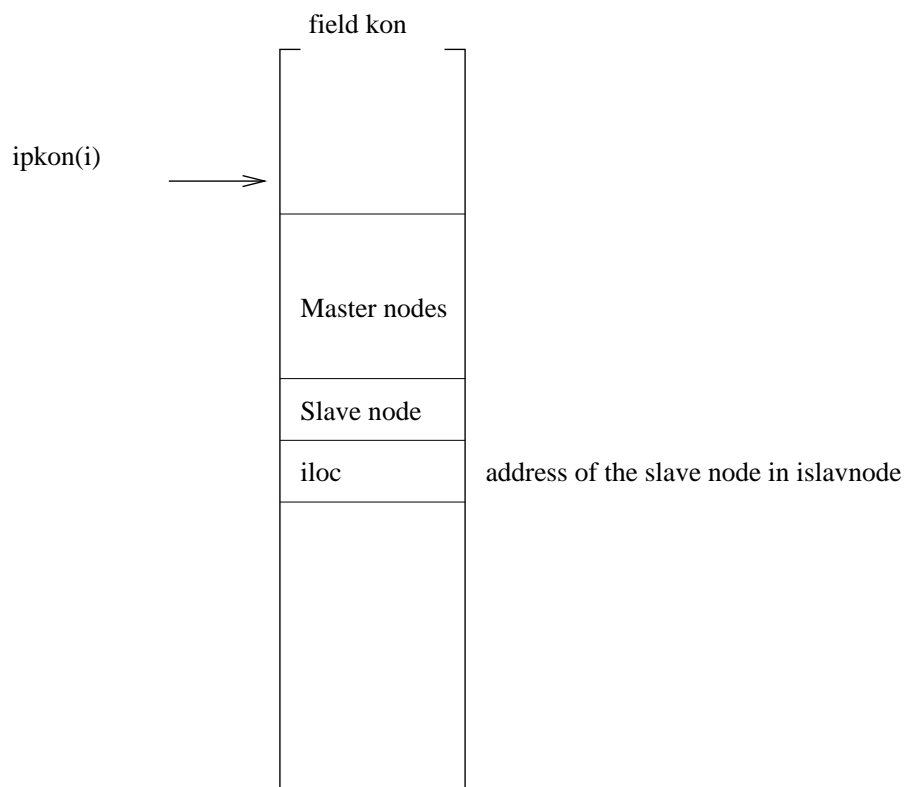
Figure 181: Topology of the node-to-face contact elements
