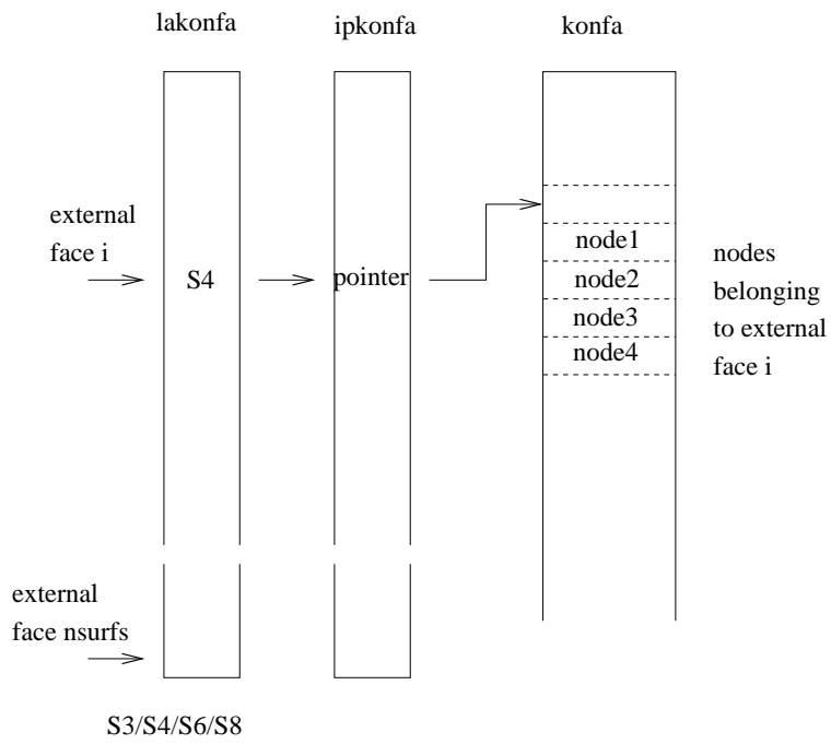
Figure 189: Data structure storing the kind of external face and the nodes belonging to that face
