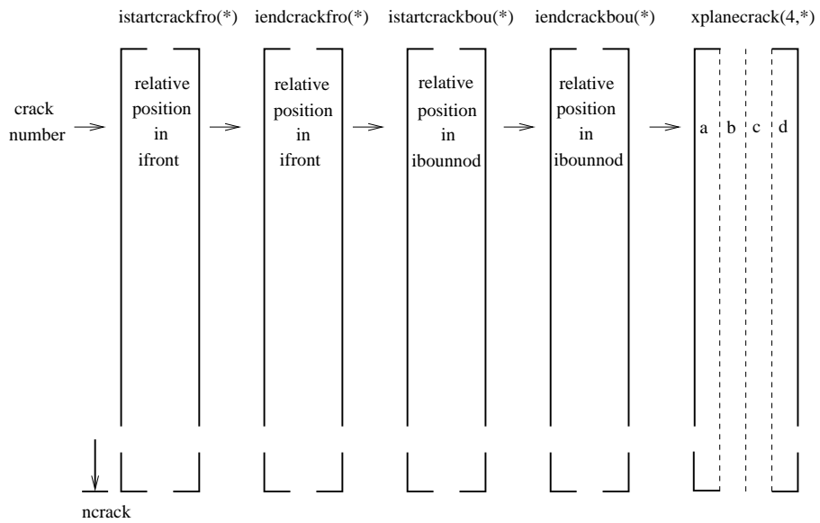
Figure 206: Fields for the crack characteristics
