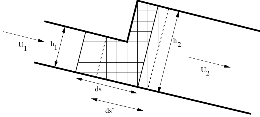
Figure 148: Conservation of momentum at a jump
