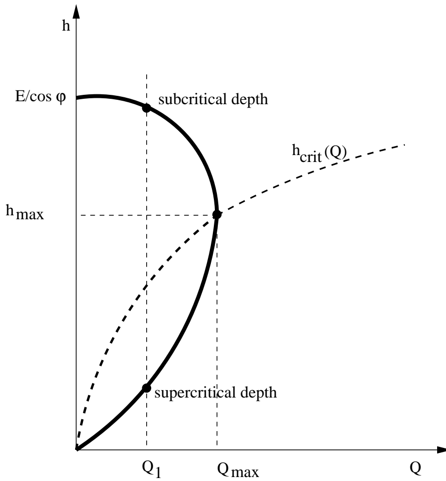
Figure 149: Allowable volumetric flow for a given specific energy
