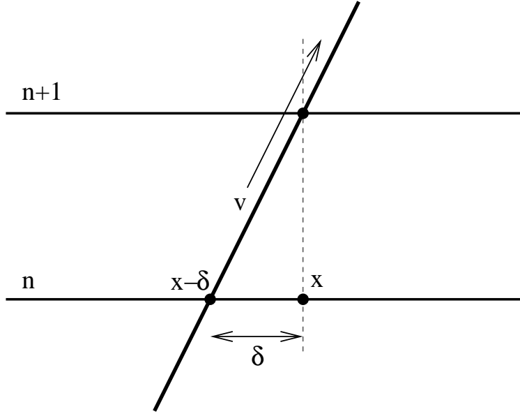
Figure 150: Formulating the equations along characteristics
