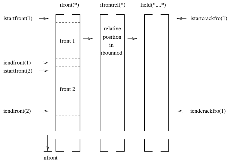
Figure 204: Fields for the front nodes (after analyzing the adjacency relations)
