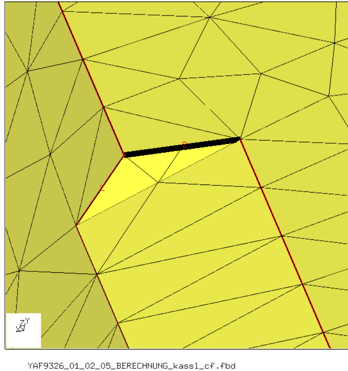
Figure 14: Visible (black) edge over lines and faces. Such edges exist if the surface mesh is not closed and not meshable with tets. Here two elements meet just one element at the black edge.
